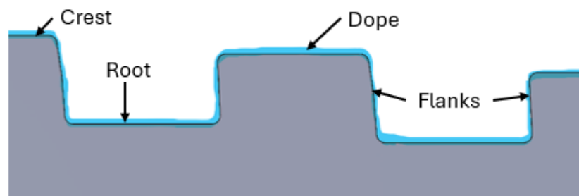
Figure 2 – Thread Form
