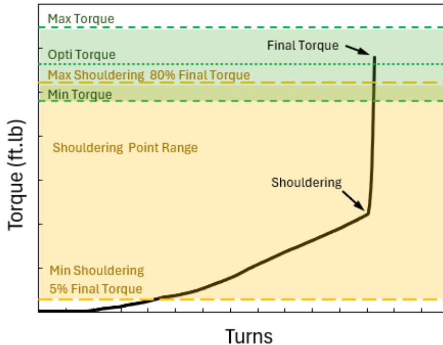
Figure 5 – Ares™ EUE Torque-Turn Signature
